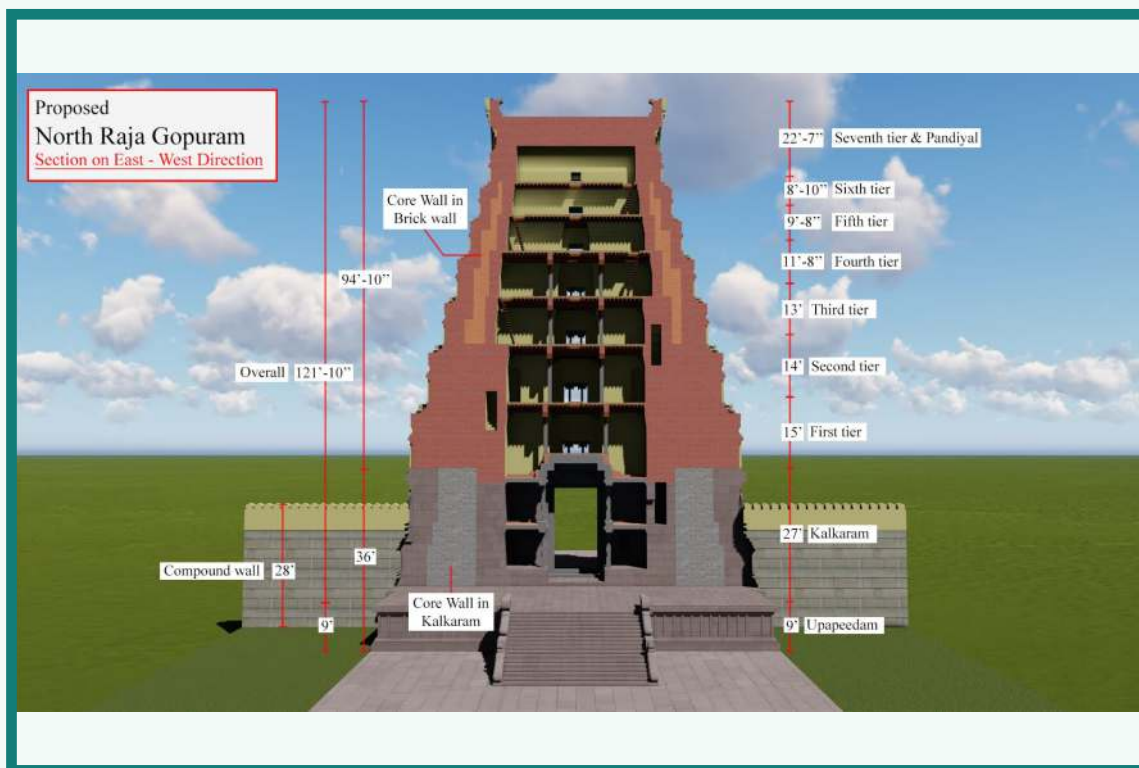
The computer generated 3D Drawings of the seven Tier completed RajaGopuram. The inside construction details are also shown.
